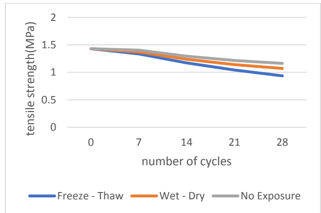
Figure 3 Comparative analysis of the effect of Sulphates on tensile strength under different exposure environments using OPC specimens.
