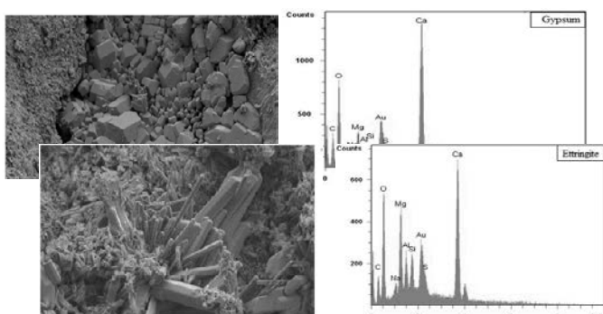
Figure 12 OPC specimens after 28 days of dipping in 3.5% concentrated solution.
